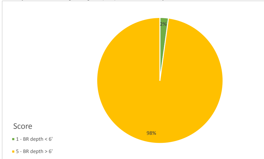
FIGURE 4 Depth to Bedrock Score Distribution Scores of 1 to 5 with 5 being the highest (best) score, see Table 2 for details
