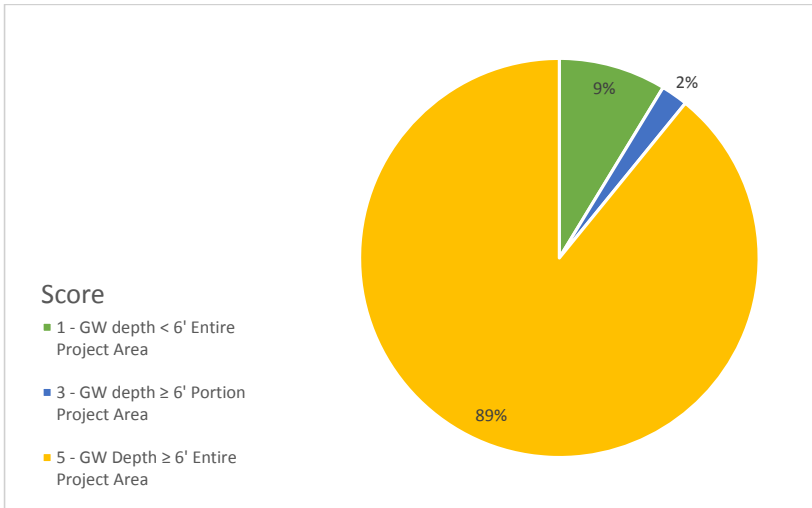
FIGURE 3 Depth to Groundwater Score Distribution Scores of 1 to 5 with 5 being the highest (best) score, see Table 2 for details
